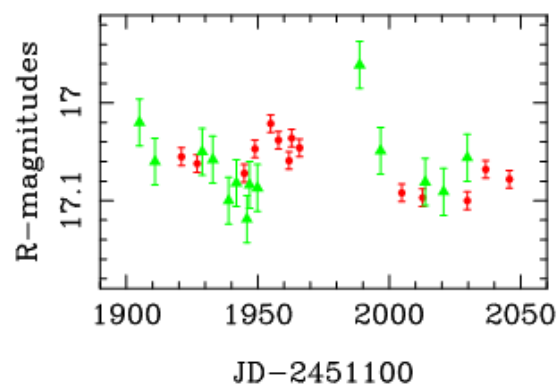
Fig. 3 Light curves of the components A and B, shifted by time and magnitude.
