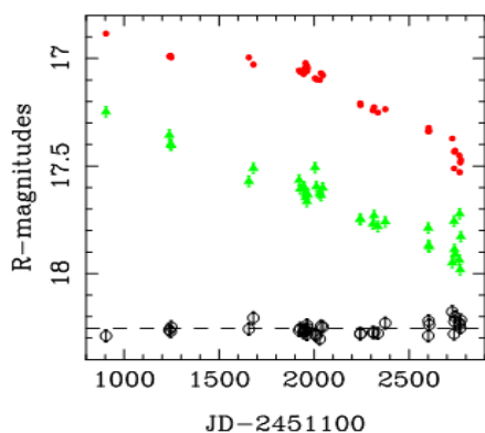
Fig. 2 Light curves of GLQ FBQ 0951+2635. From top to bottom - components A and B, as well as the reference star.
