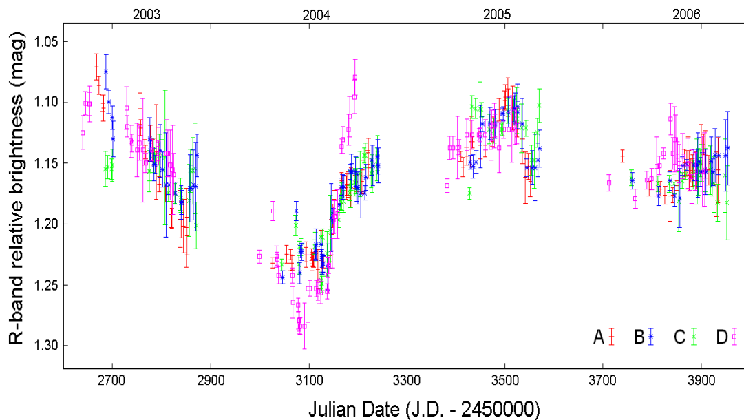
Fig. 10 Light curves of the lensed components A, B, C and D in the R-band with taking into account the our time delays.
