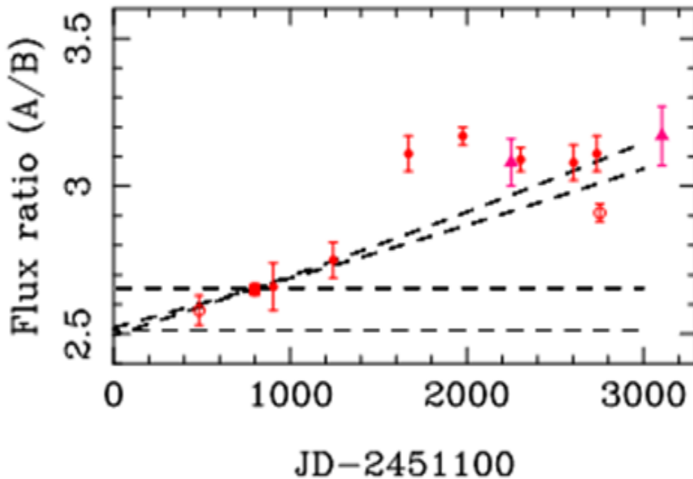
Fig.4 Variation of the flux ratio between components of the GLQ FBQ 0951+2635 versus time in the optic band.
